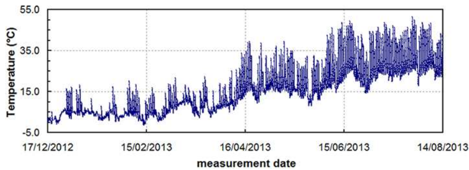
Fig. 8. Outdoor temperature measured on S-W front in the period between 17/12/2012 and 13/08/2013
