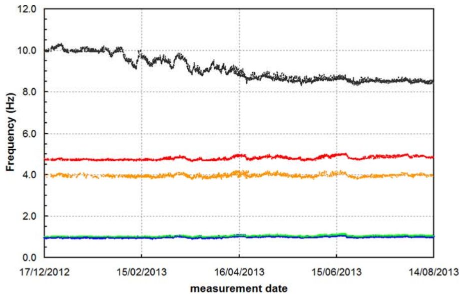
Fig. 9. Variation of the automatically identified (SSI-Cov) natural frequencies in the period between 17/12/2012 and 13/08/2013
