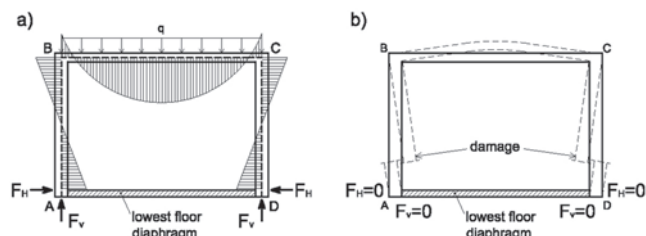
Fig. 23. During the downwards motion phase, the structure, designed to carry mainly gravitational loads, is suddenly in a space condition without gravity; a) the case with gravity; b) the existing frame is without gravity.
