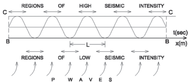
Fig. 17. Ground motion in the epicentral regions (where the vertical earthquake motion dominates): in B-B is the surface of the ground at its initial position; in C-C is the extreme position of the ground due to P waves and the vertical projection of R wave particle motion; B-C compressional field is the vertical projection of the final motion of the ground particles; L is the wave length of surface waves.
