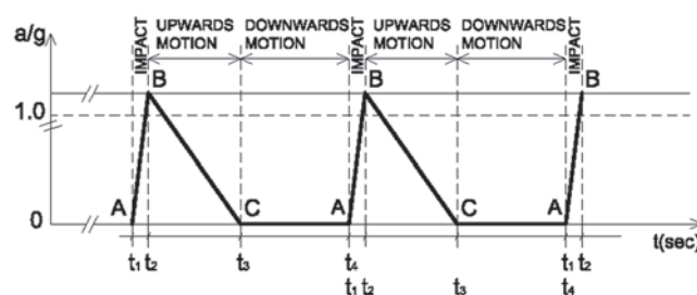
Fig. 21. Accelerations created on the center of mass of a structure elastically jumping on the ground due to the vertical earthquake component: A-B, \Delta t_1 = t_2 - t_1 impact phase; B, t_2 detachment from the ground; B-C, \Delta t_2 = t_3 - t_2 upwards motion, up to the highest position at C; C-A, \Delta t_3 = t_4 - t_3 , zero acceleration during its downwards motion (the structure is in a space without gravity!).
